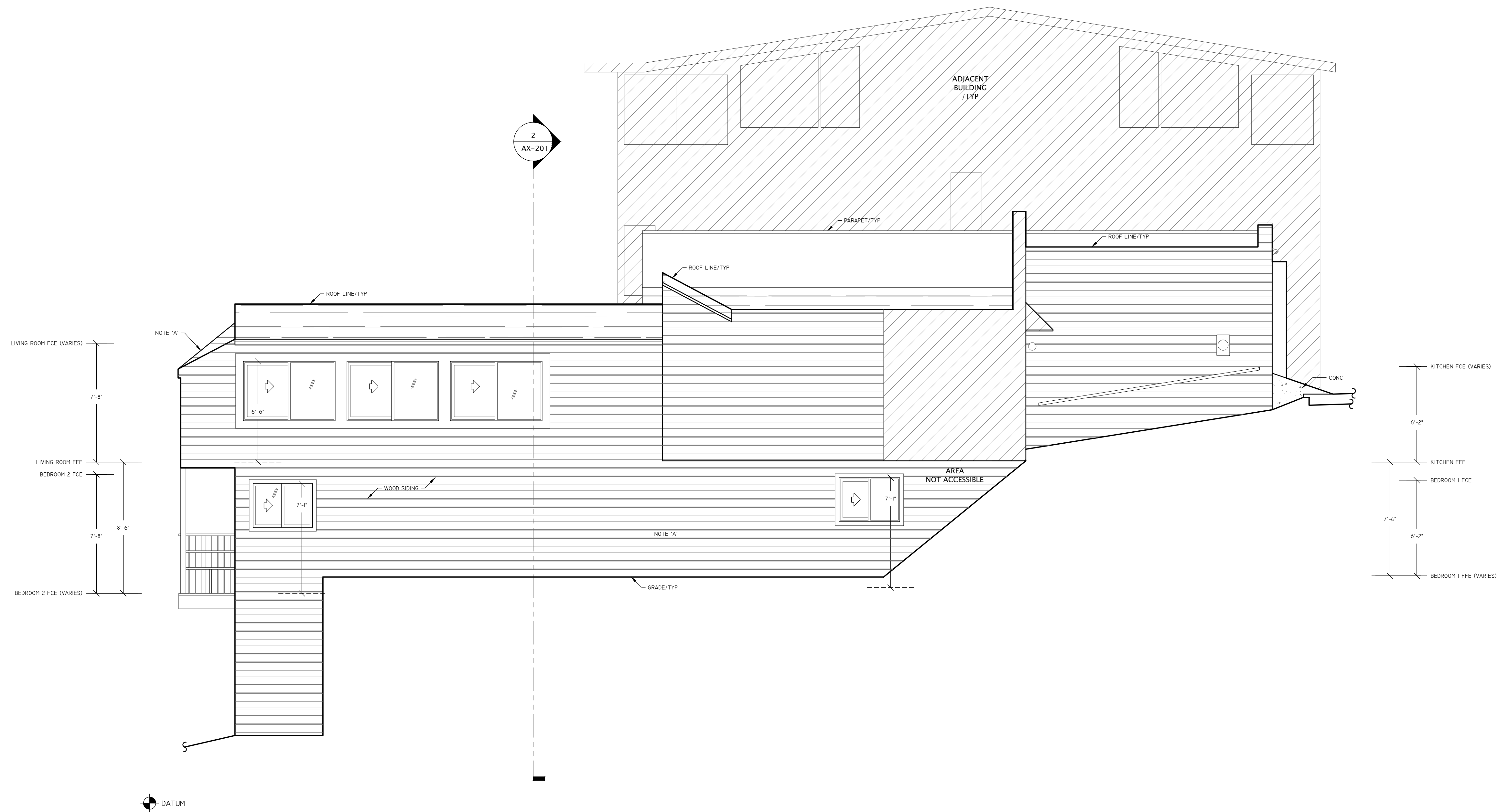
1 EXISTING NORTH ELEVATION
