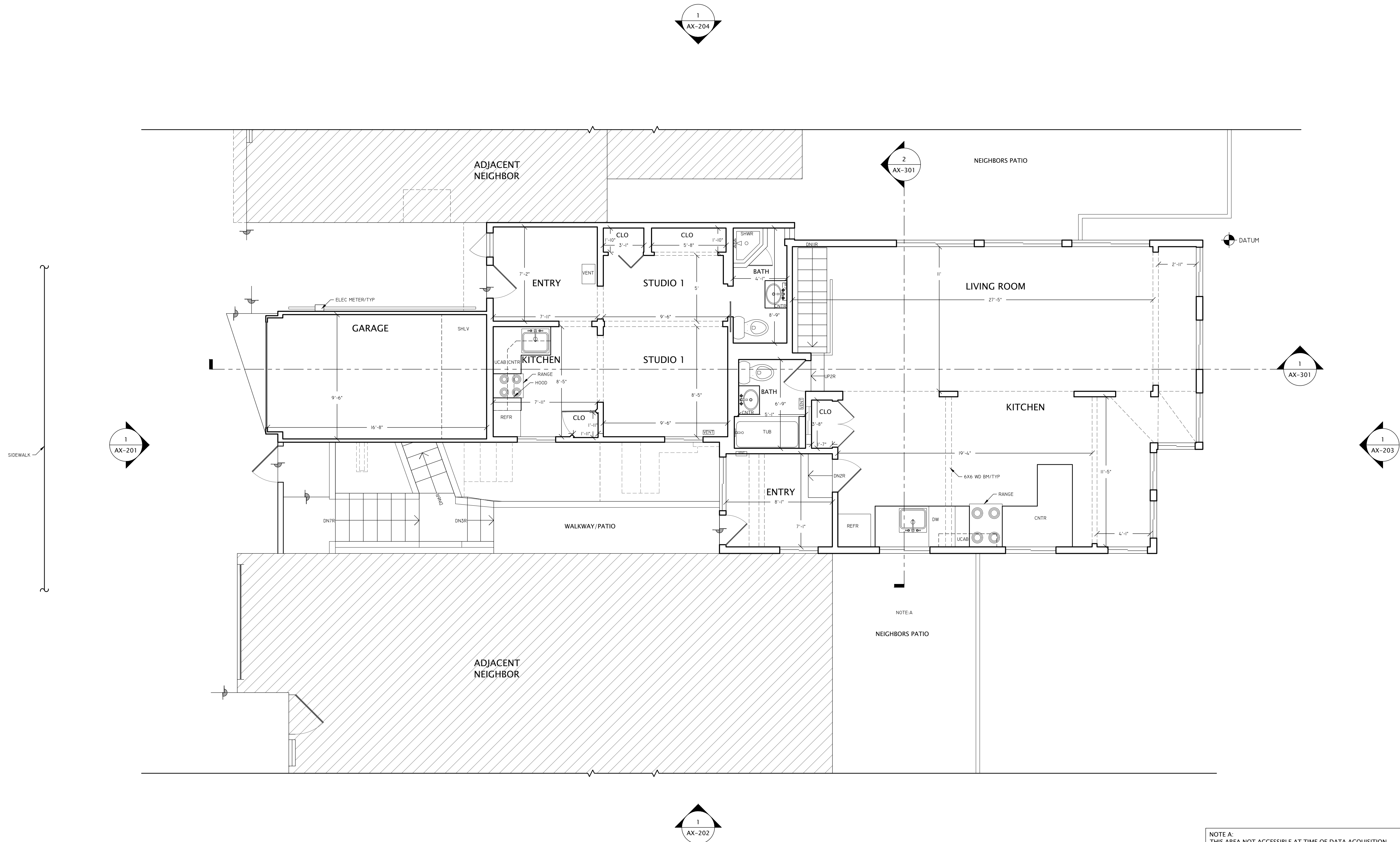
1 EXISTING ENTRY LEVEL FLOOR PLAN 1,318 SQFT GROSS MEASURED AREA 284 SQFT MEASURED EXTERIOR SURFACES
